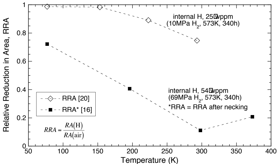
Figure 3.1.1.2. Relative reduction of area (RRA) of smooth tensile specimens of JBK-75 stainless steel as a function of temperature; with internal hydrogen (measured in air after thermal precharging in hydrogen gas). Data from Ref. [20] is also presented in Table 3.1.1.3 and Figure 3.1.1.1.
